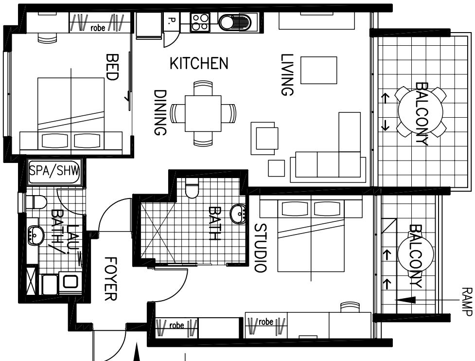
APARTMENT TYPE B1 DISABLED – LEVEL 2
